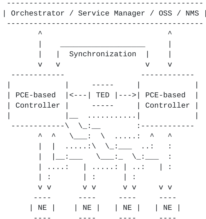
Figure 5: Multiple Redundant Controllers
