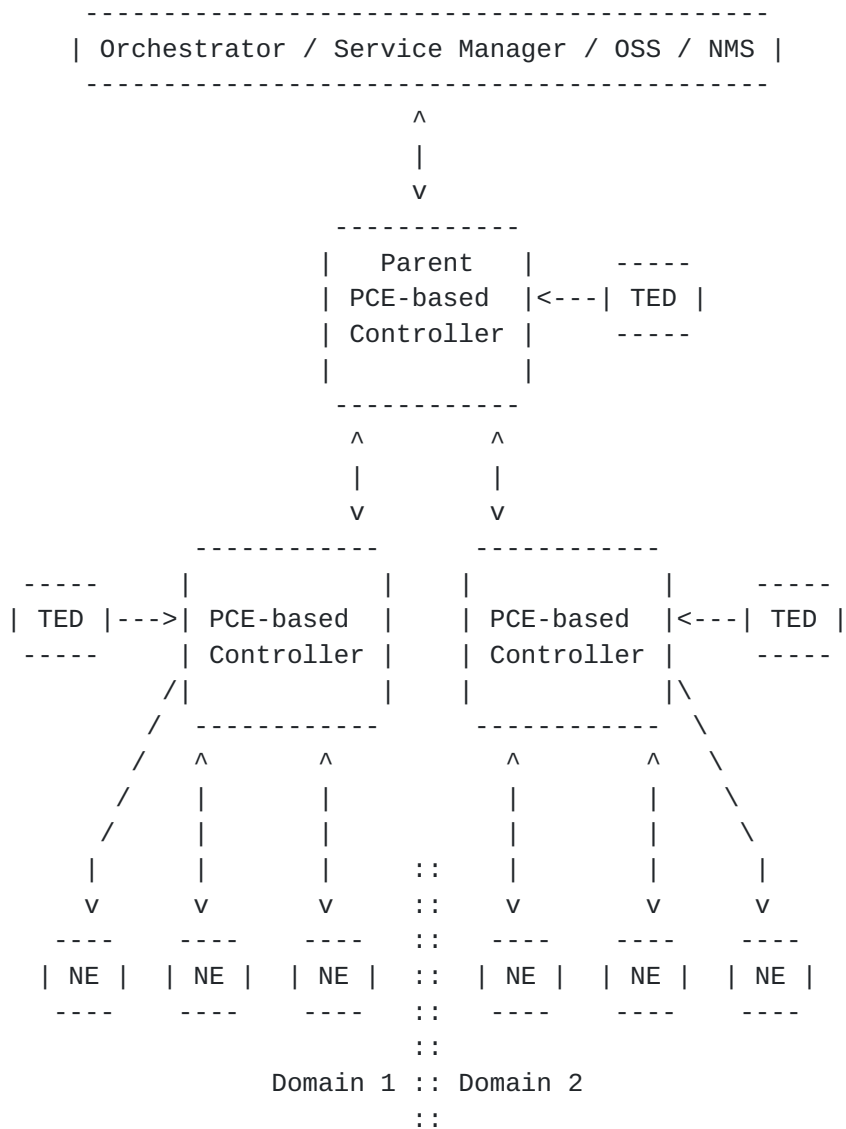
Figure 6: Hierarchical Controllers
