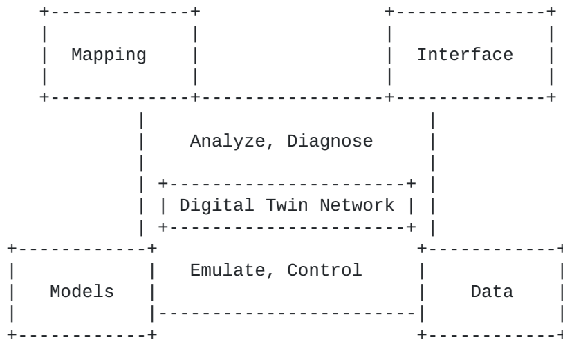
Figure 1: Key Elements of Digital Twin Network
