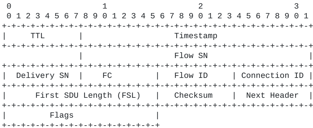
Figure 4: GMA Trailer Format
