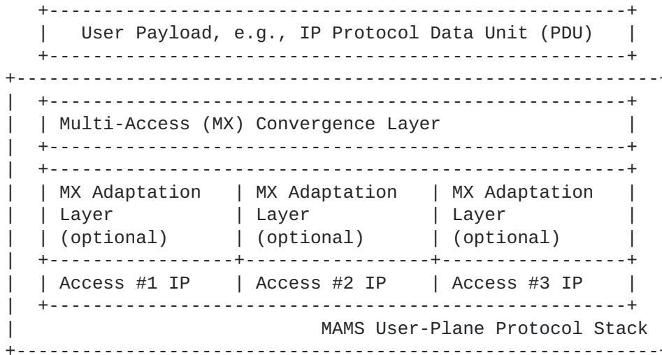
Figure 1: MAMS User-Plane Protocol Stack [ MAMS ]
