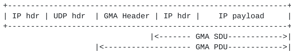
Figure 7: GMA PDU Format with Non-IP Encapsulation
