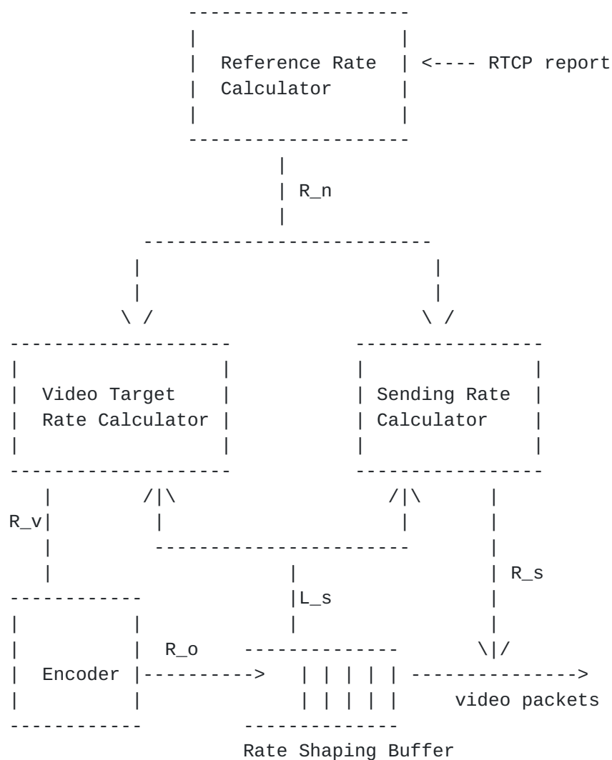
Figure 1 NADA Sender Structure
