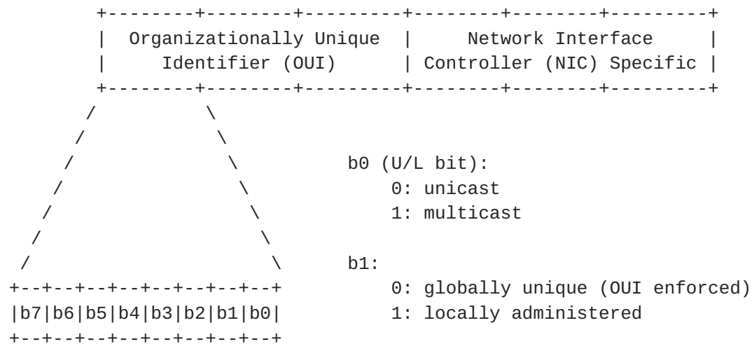
Figure 1: IEEE 802 MAC Address Format
