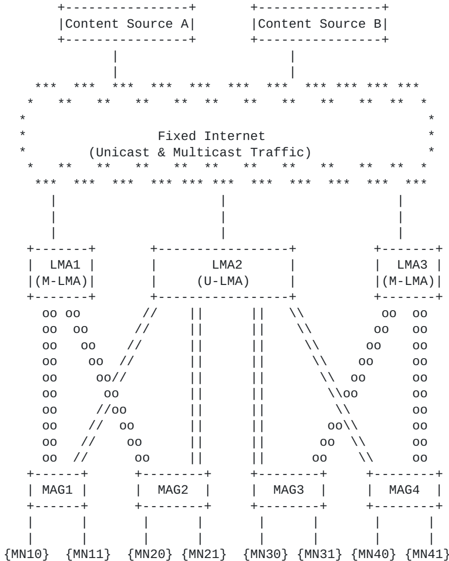
Figure 3. PMIPv6 domain with ratio 1:N
