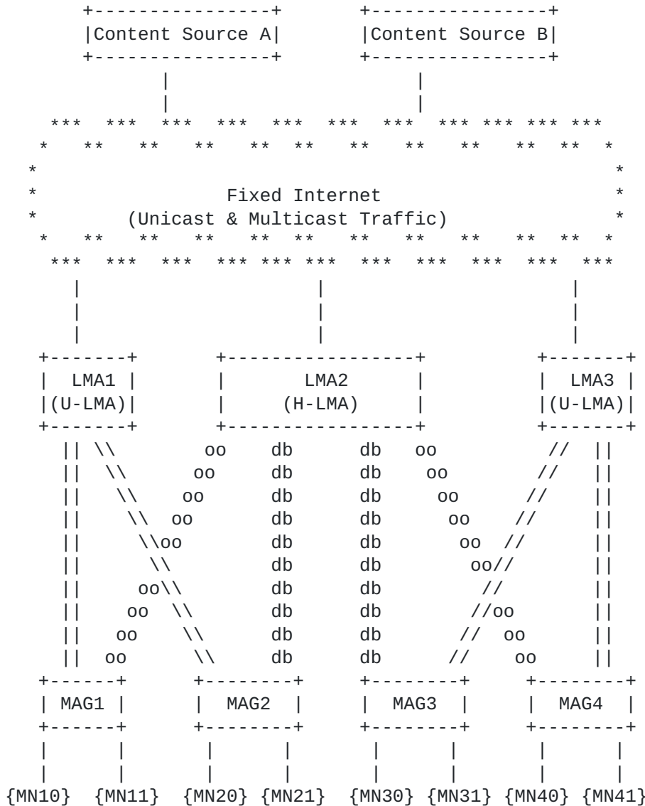
Figure 4. PMIPv6 domain with H-LMA
