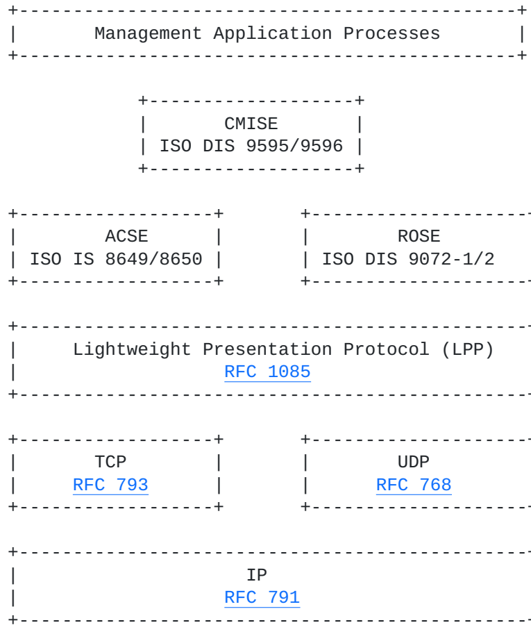
Figure 2. The CMOT Protocol Suite
