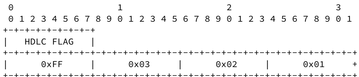
Figure 4: Bridge "Hello" PDU
