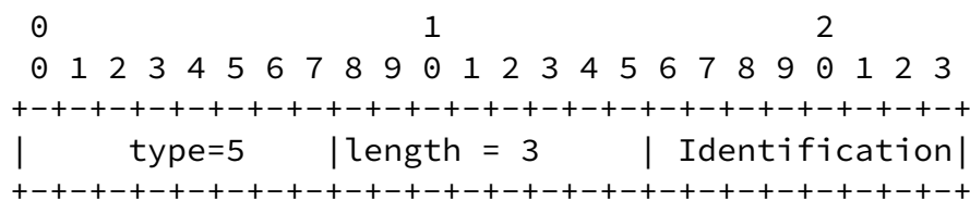
Figure 9: LAN Identification Option
