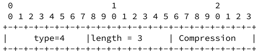
Figure 8: Tinygram Compression Option
