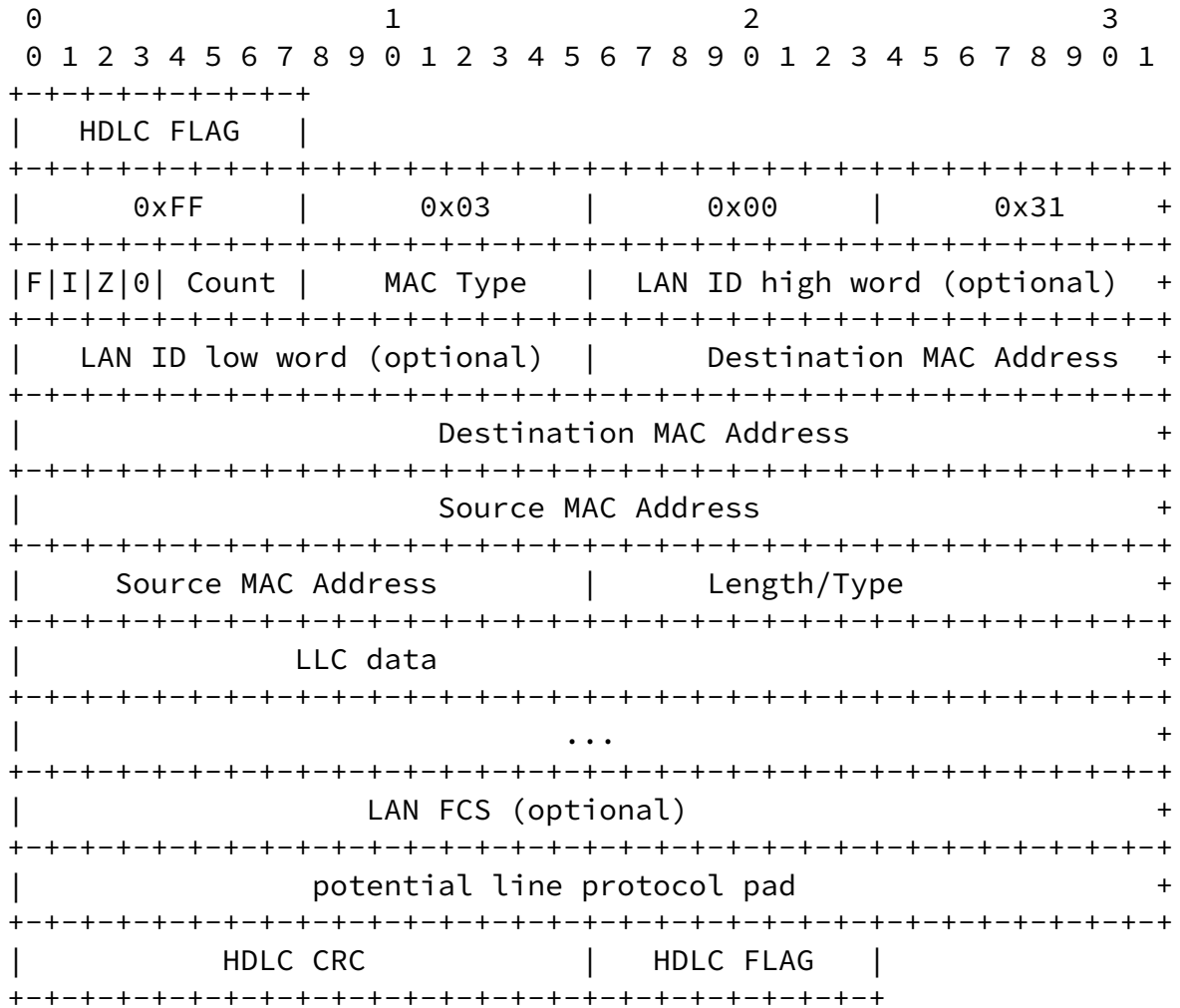
Figure 2: 802.3 Frame format
