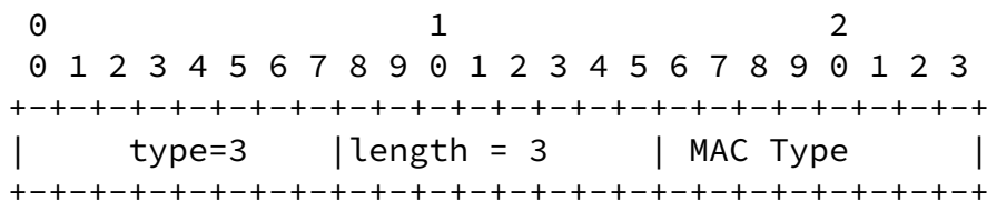
Figure 7: MAC Type Selection Option
