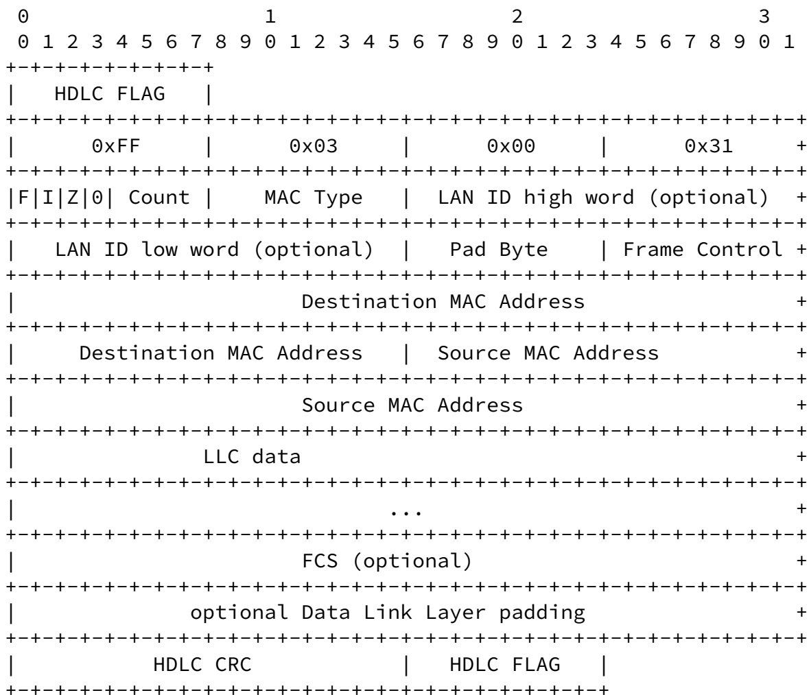
Figure 3: 802.4/802.5/FDDI Frame format
