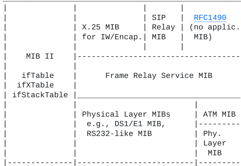
Figure 1. Frame Relay MIB Architecture
