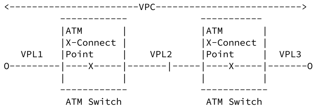
Figure 2: Virtual Path Links and Virtual Path Connection
