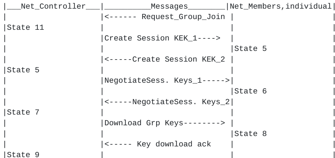
Figure 4: State Diagram: Member Join
