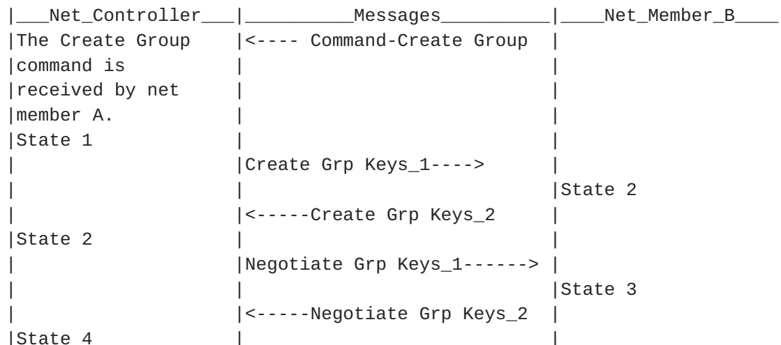
Figure 1: State Diagram: Create Group Keys
