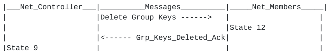
Figure 5: State Diagram: Cooperative Delete
