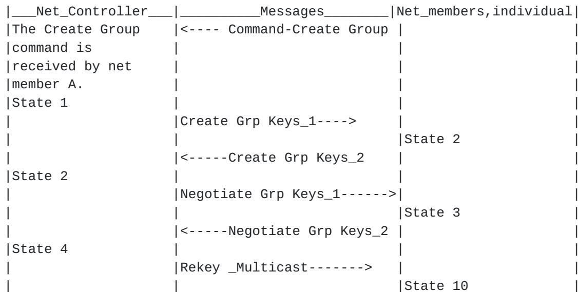
Figure 3: State Diagram: Rekey
