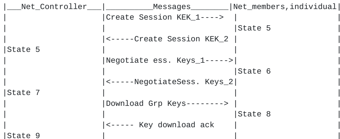
Figure 2: State Diagram: Distribute Keys
