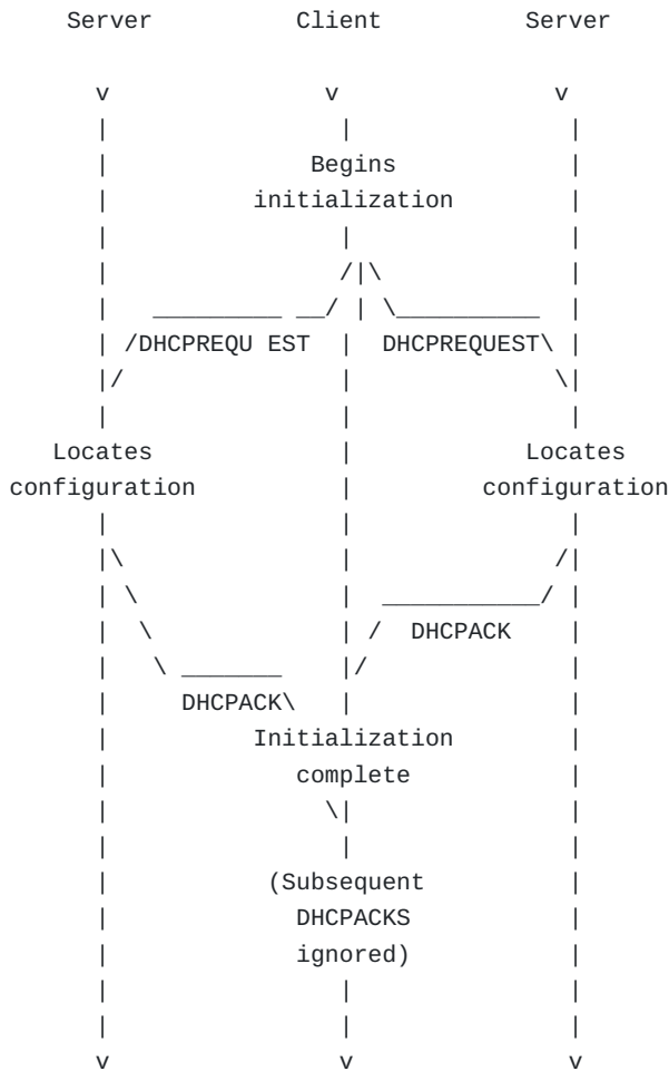
Figure 4: Timeline diagram of messages exchanged between DHCP client and servers when reusing a previously allocated network address
