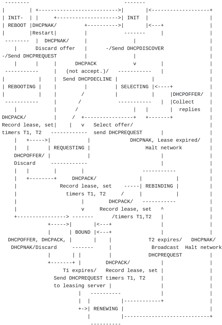
Figure 5: State-transition diagram for DHCP clients
