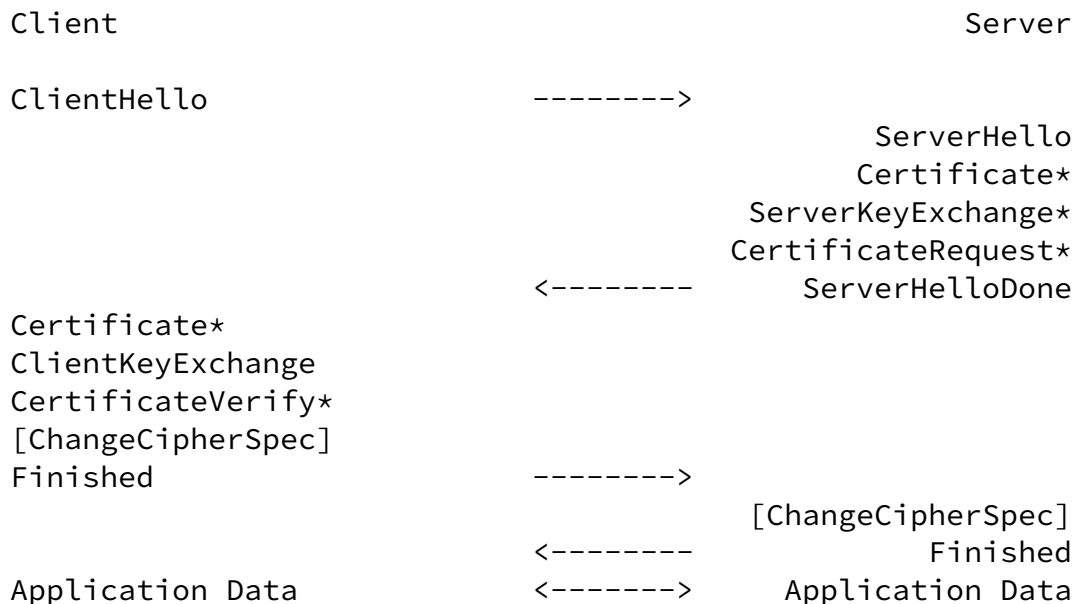
Fig. 1 - Message flow for a full handshake
