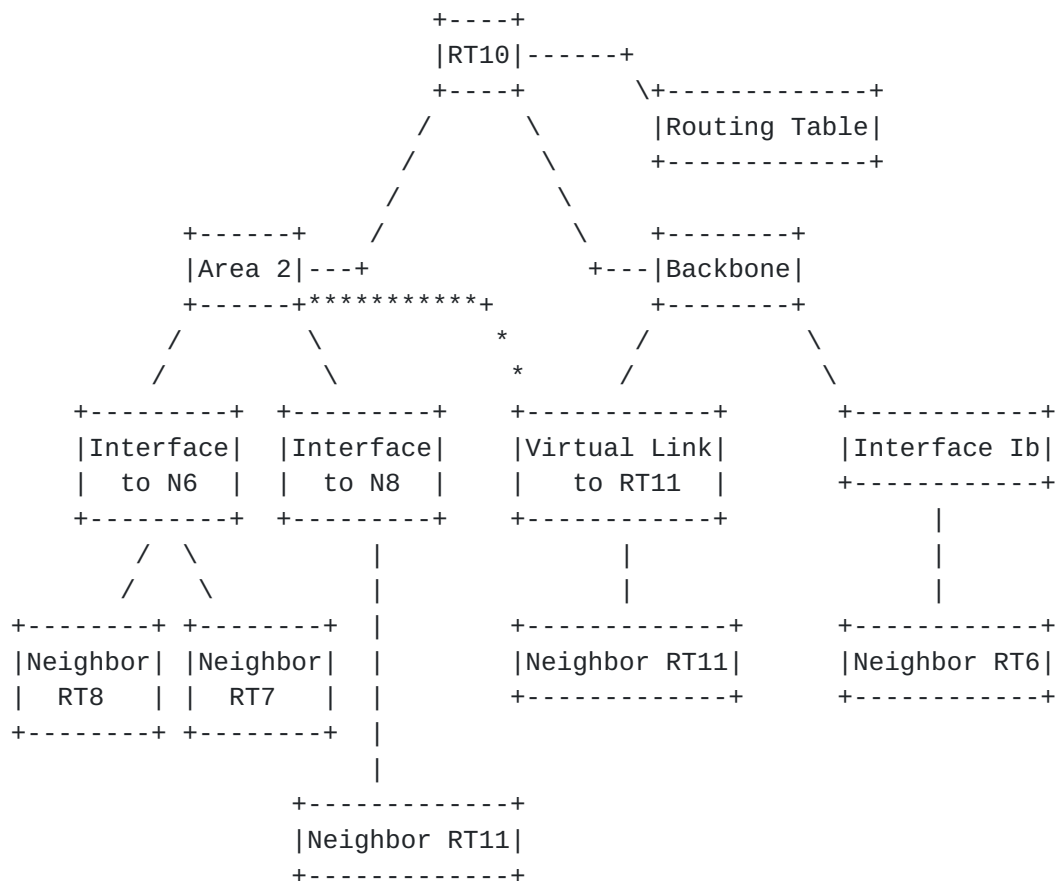
Figure 9: Router RT10's Data structures
