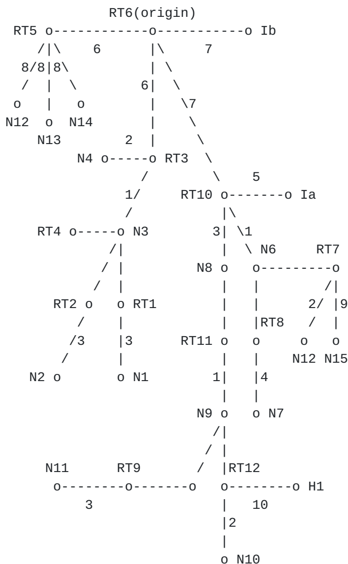
Figure 5: The SPF tree for Router RT6
