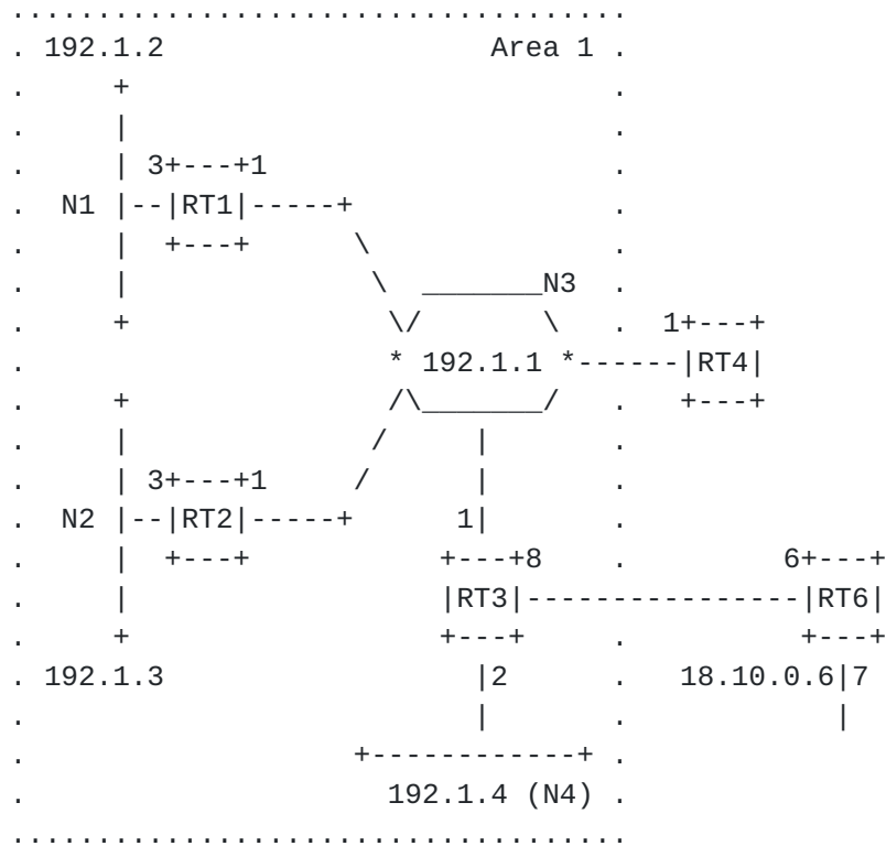
Figure 15: Area 1 with IP addresses shown
