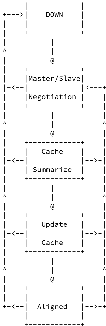
Figure 2: Cache Alignment Finite State Machine
