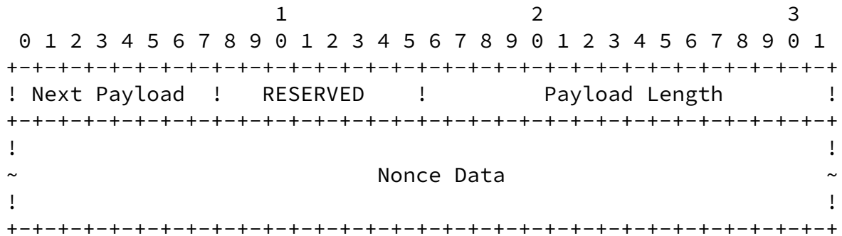
Figure 14: Nonce Payload Format
