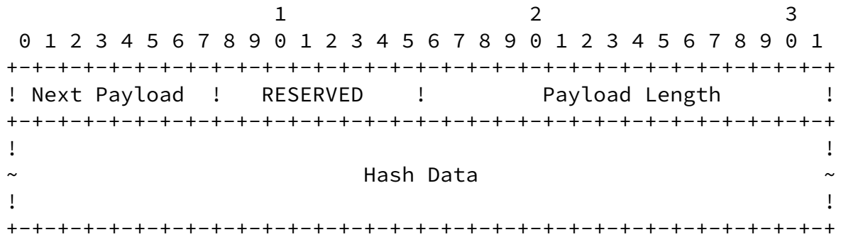
Figure 12: Hash Payload Format
