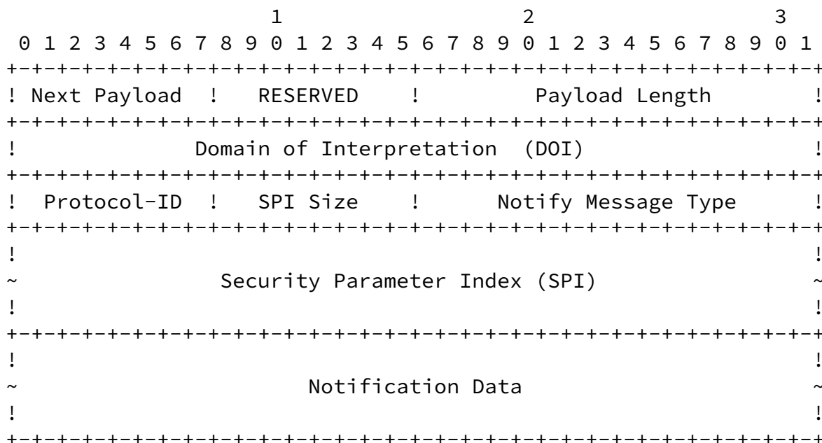
Figure 15: Notification Payload Format
