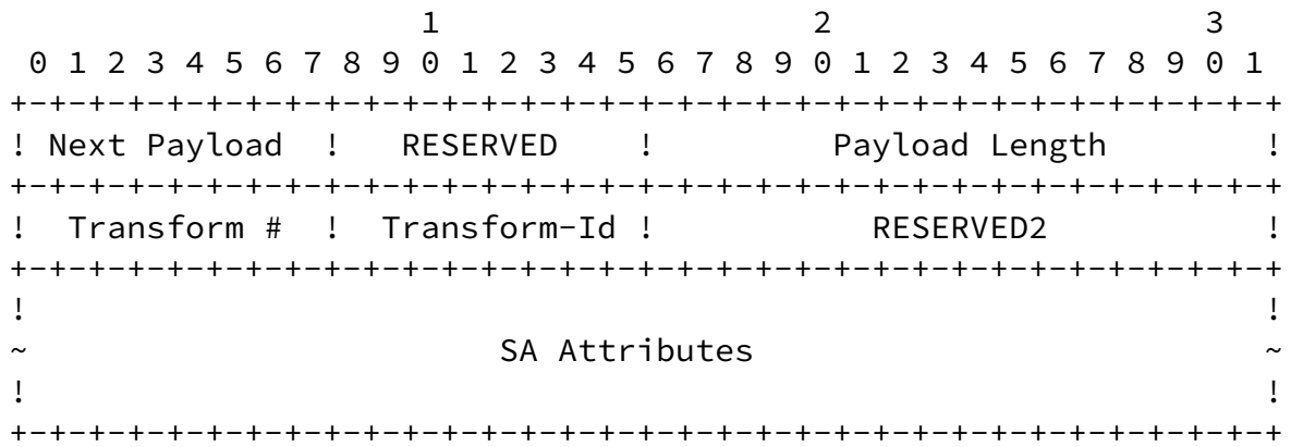
Figure 7: Transform Payload Format
