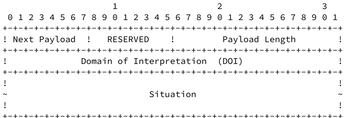
Figure 5: Security Association Payload
