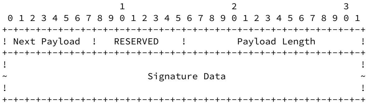
Figure 13: Signature Payload Format
