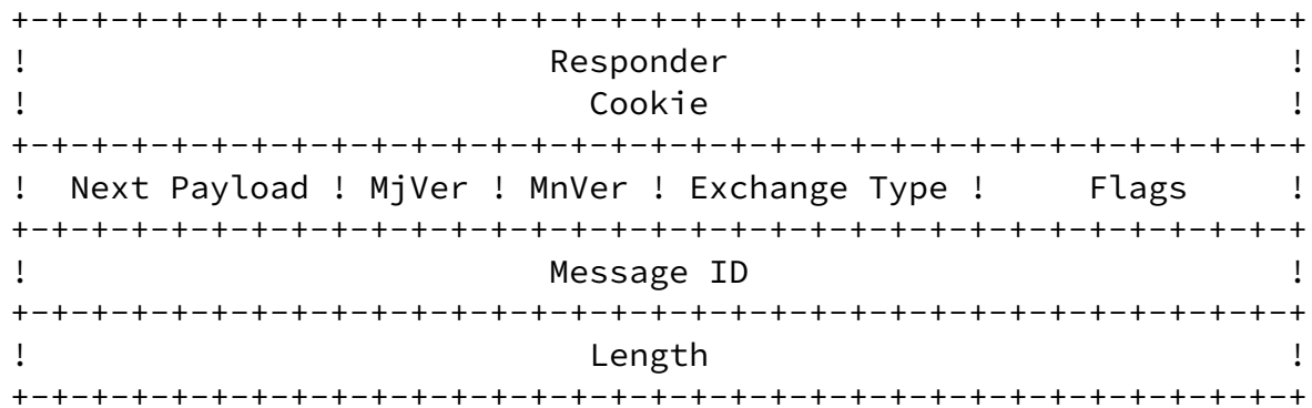
Figure 2: ISAKMP Header Format
