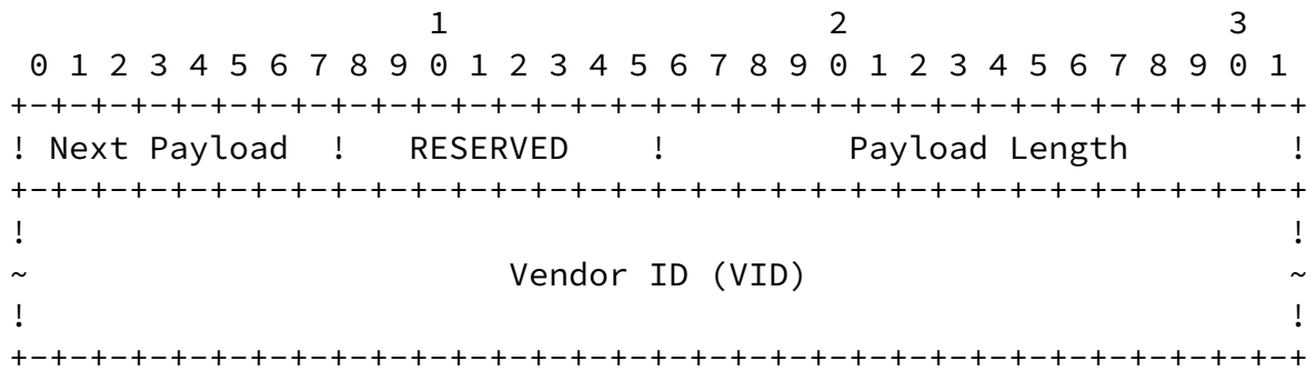
Figure 17: Vendor ID Payload Format
