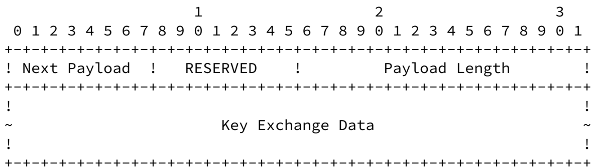
Figure 8: Key Exchange Payload Format
