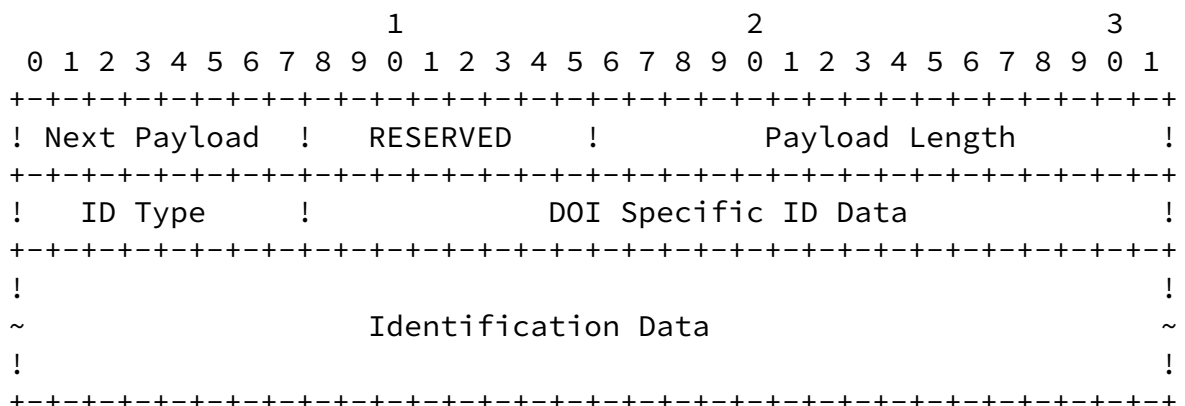
Figure 9: Identification Payload Format
