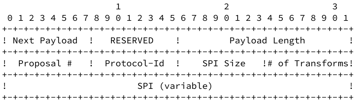
Figure 6: Proposal Payload Format
