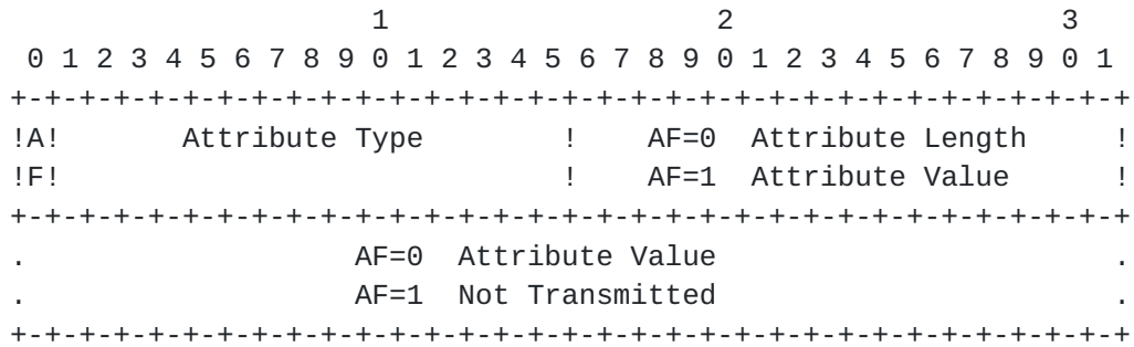
Figure 4: Data Attributes
