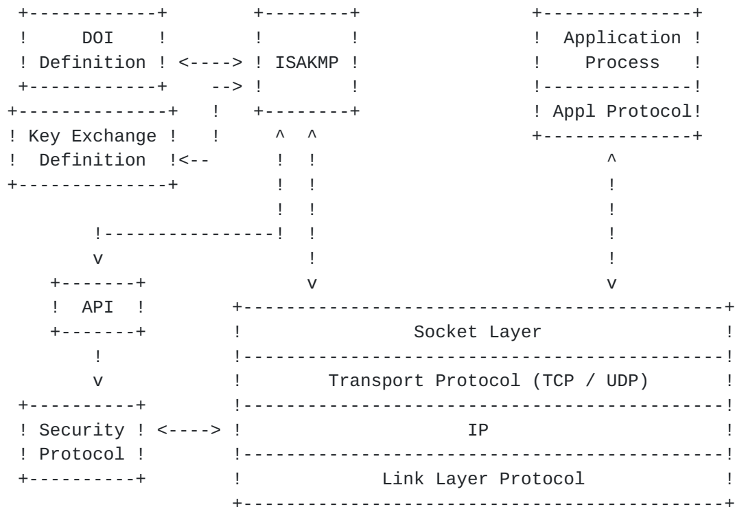
Figure 1: ISAKMP Relationships
