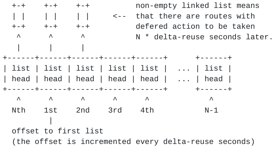
Figure 4: Reuse List Data Structures
