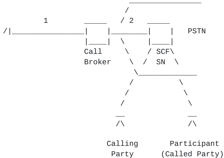
Figure 12: The CallBroker Architecture
