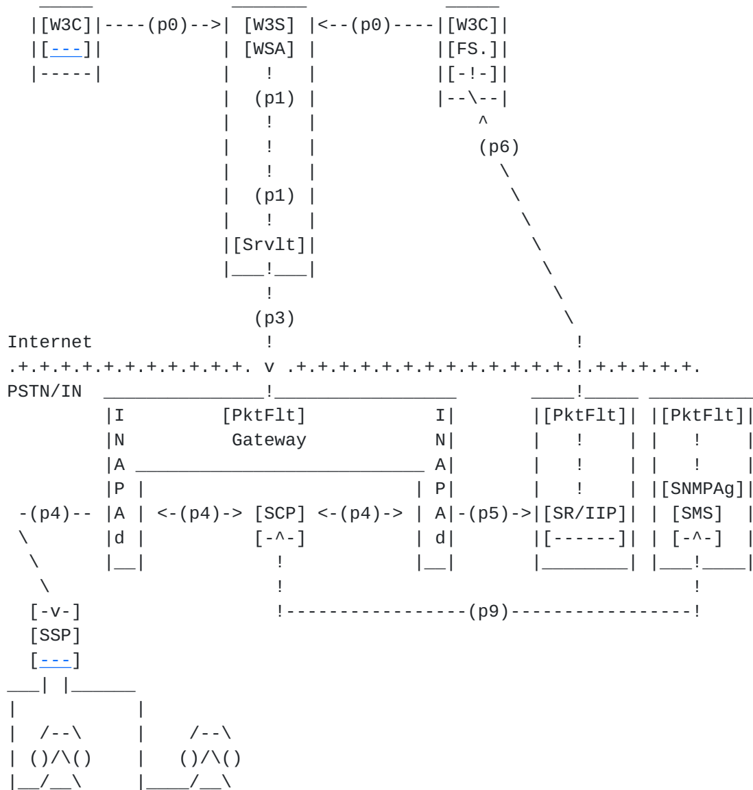
Figure 7: The Siemens Web Call Center
