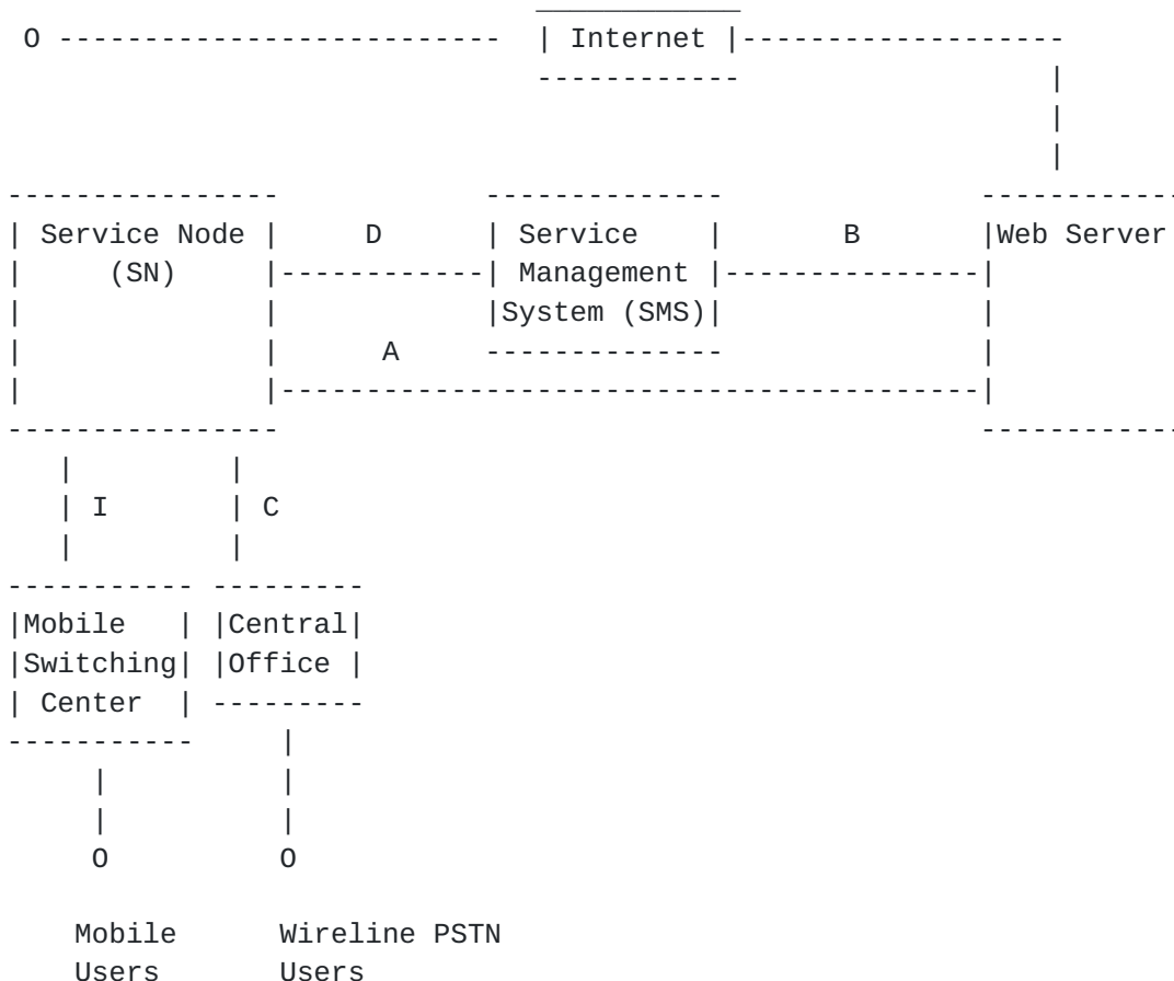
Figure 11: Overall Interconnection Architecture of the Lucent System
