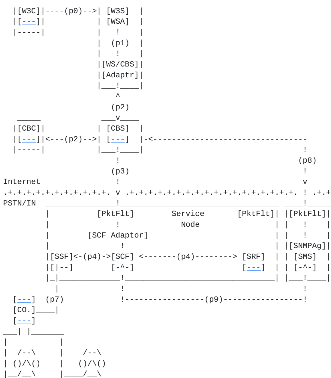
Figure 9: The AT&T System
