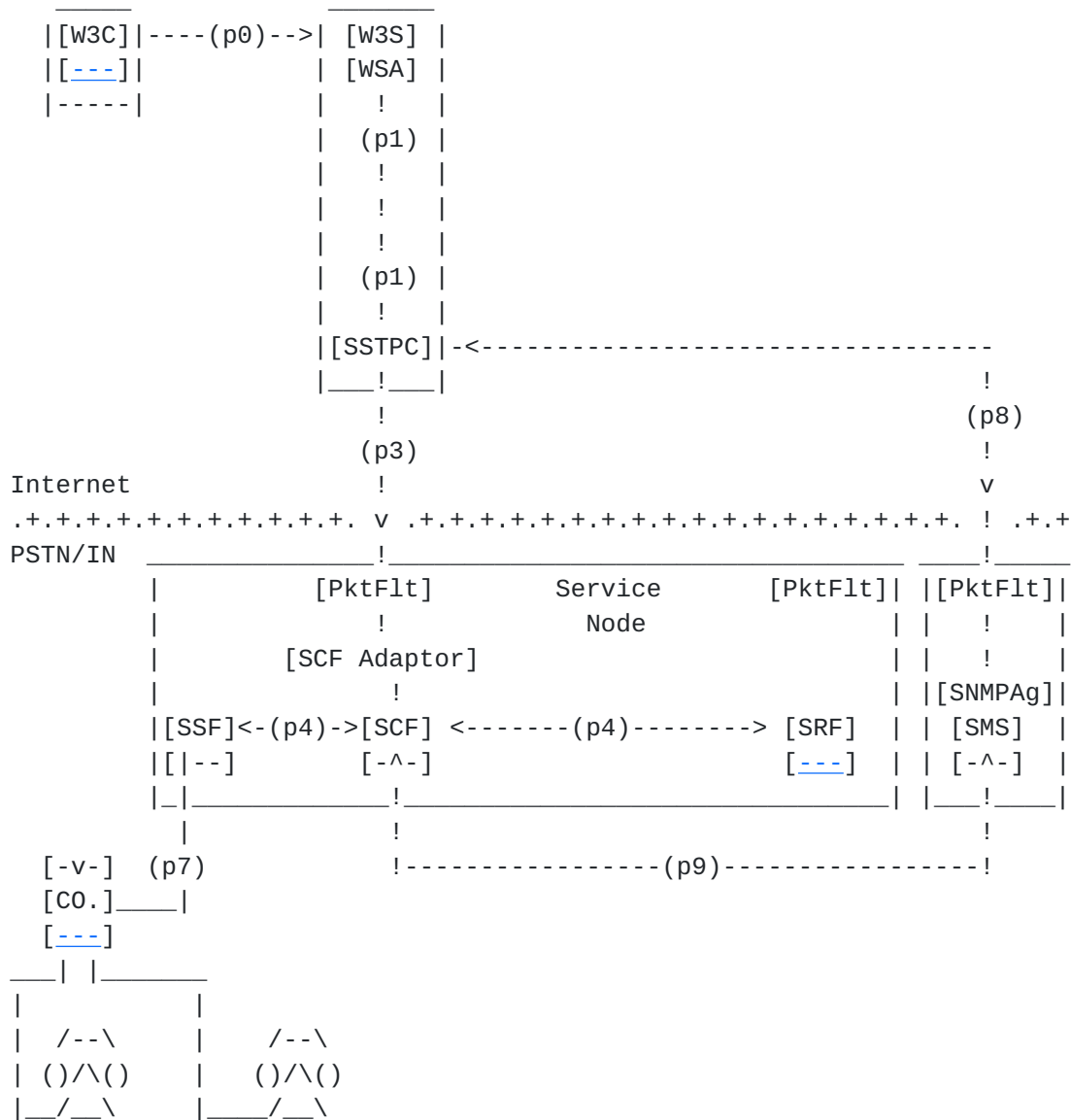
Figure 8: The Lucent System
