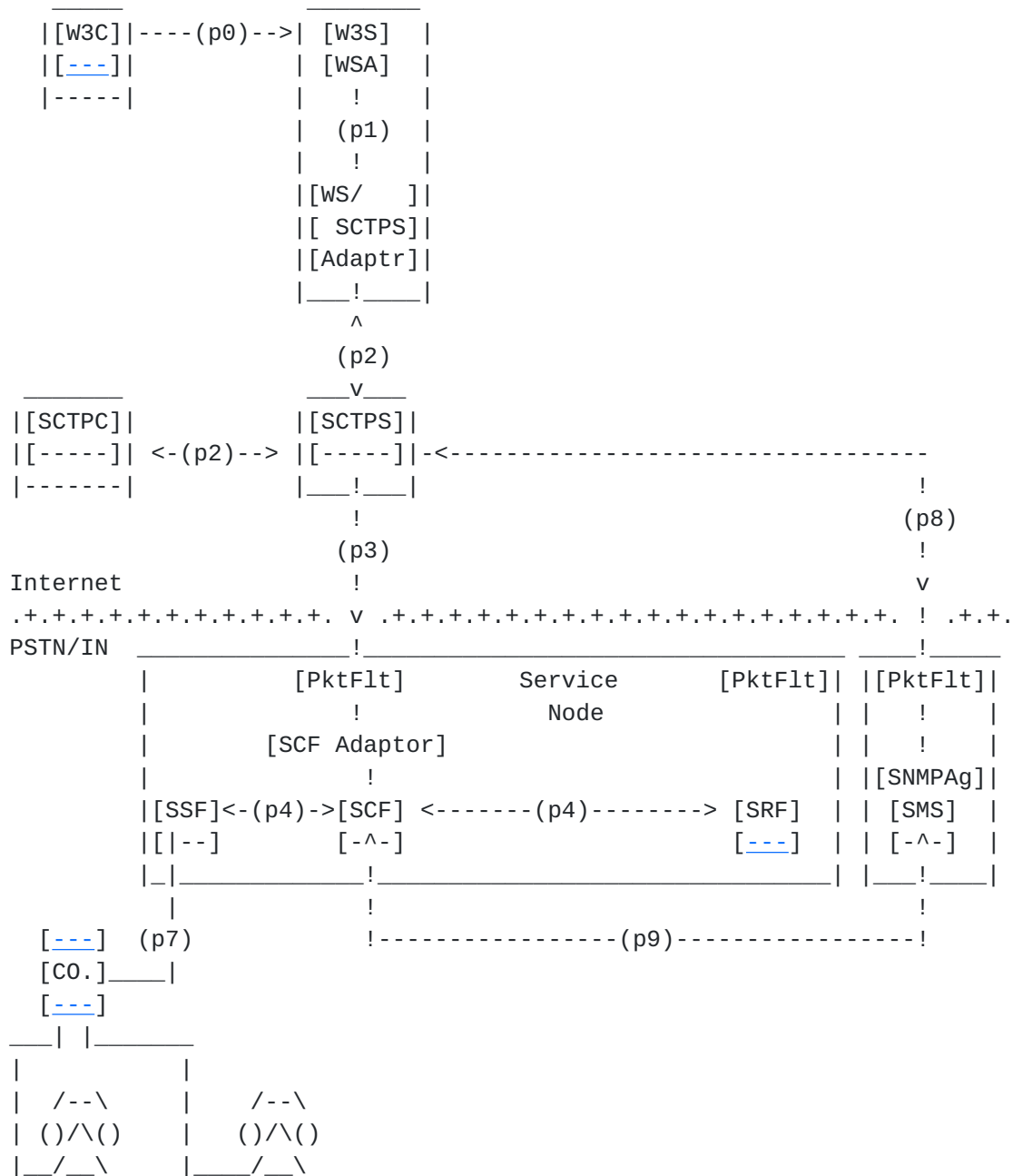
Figure 10: The Nortel System
