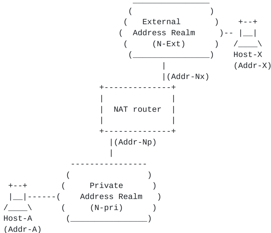
Figure 2: A base model to illustrate NAT terms.
