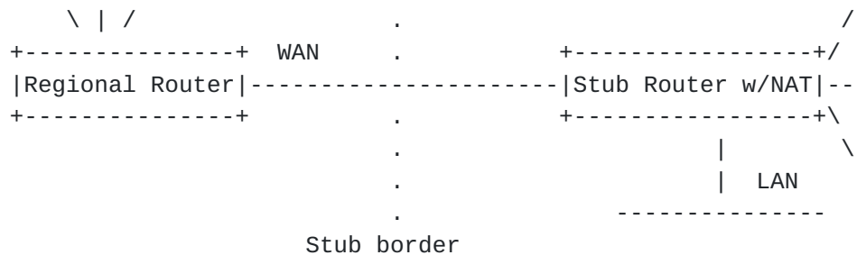
Figure 1: A typical NAT operation scenario
