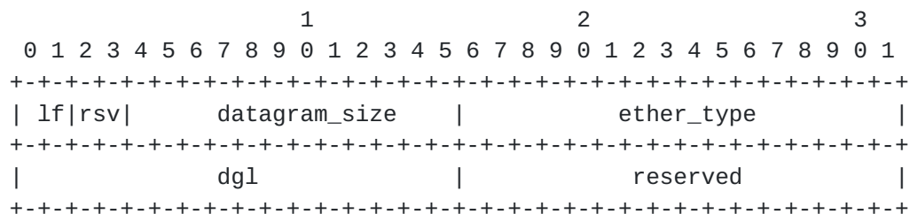
Figure 3 - First fragment encapsulation header format
