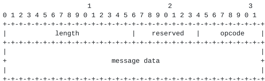
Figure 10 - MCAP message format
