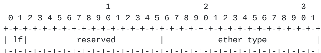
Figure 2 - Unfragmented encapsulation header format
