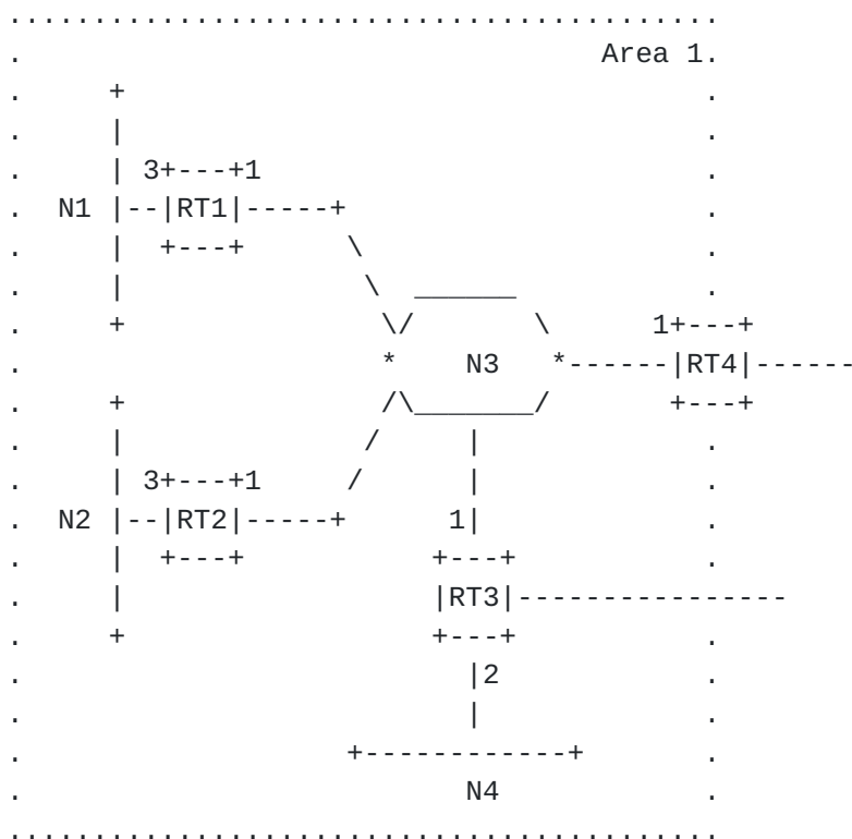
Figure 1: Area 1 with IP addresses shown
