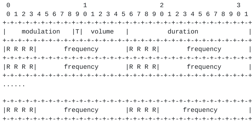
Figure 3: Payload format for tones
