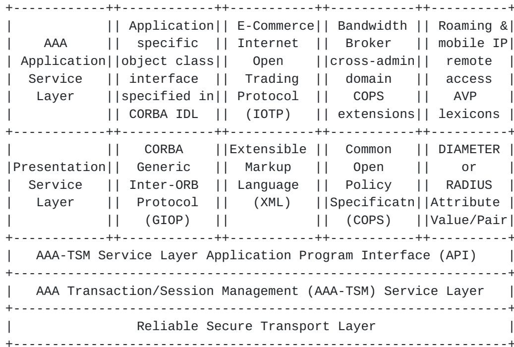
Fig. 6 -- Possible AAA Protocol Stacks
