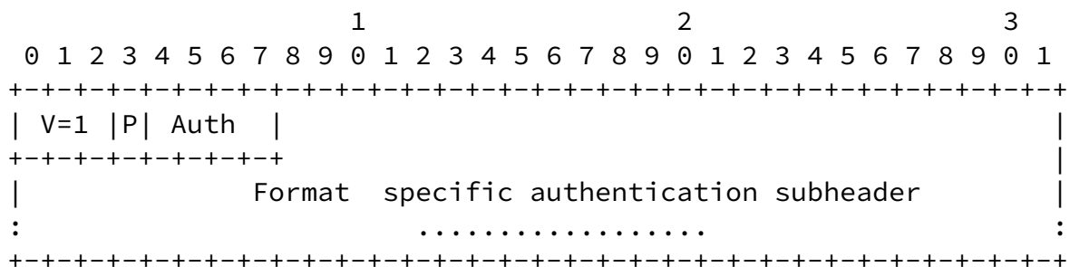
Figure 2: Format of the authentication data in the SAP header
