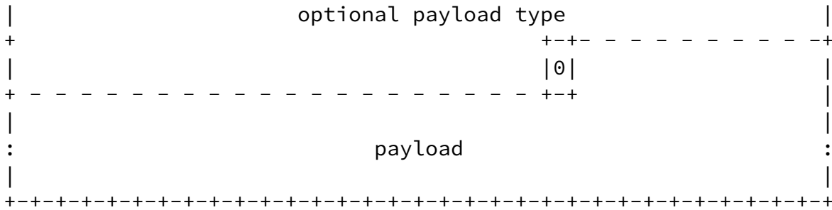
Figure 1: Packet format
