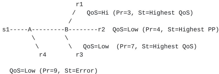
Example 1: Merging preempted priority elements
