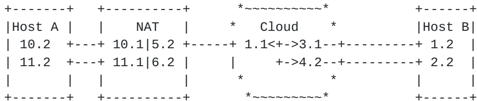
Fig 2: SCTP through NAT with multihoming
