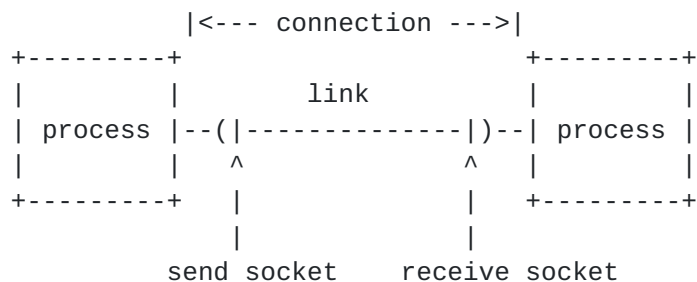
Figure 4 The relationship between sockets and processes
