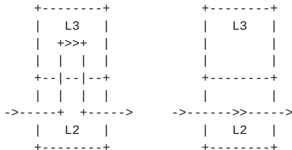
Figure 6. Unicast forwarding on resp. L3 or L2
