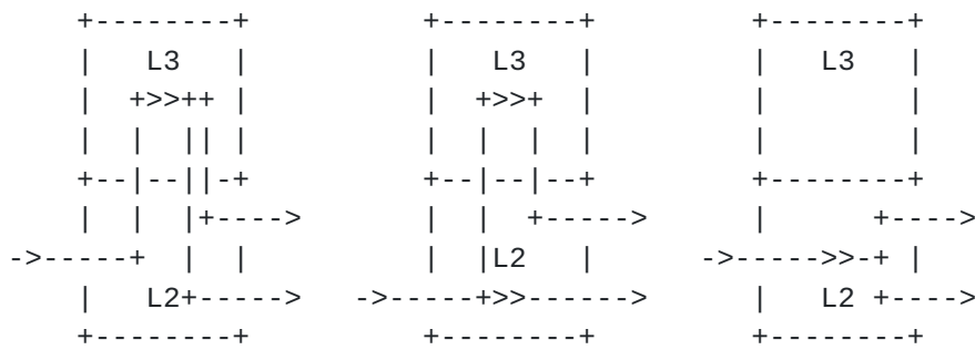
Figure 7. Multicast forwarding on resp. L3, mixed L2/L3 or L2
