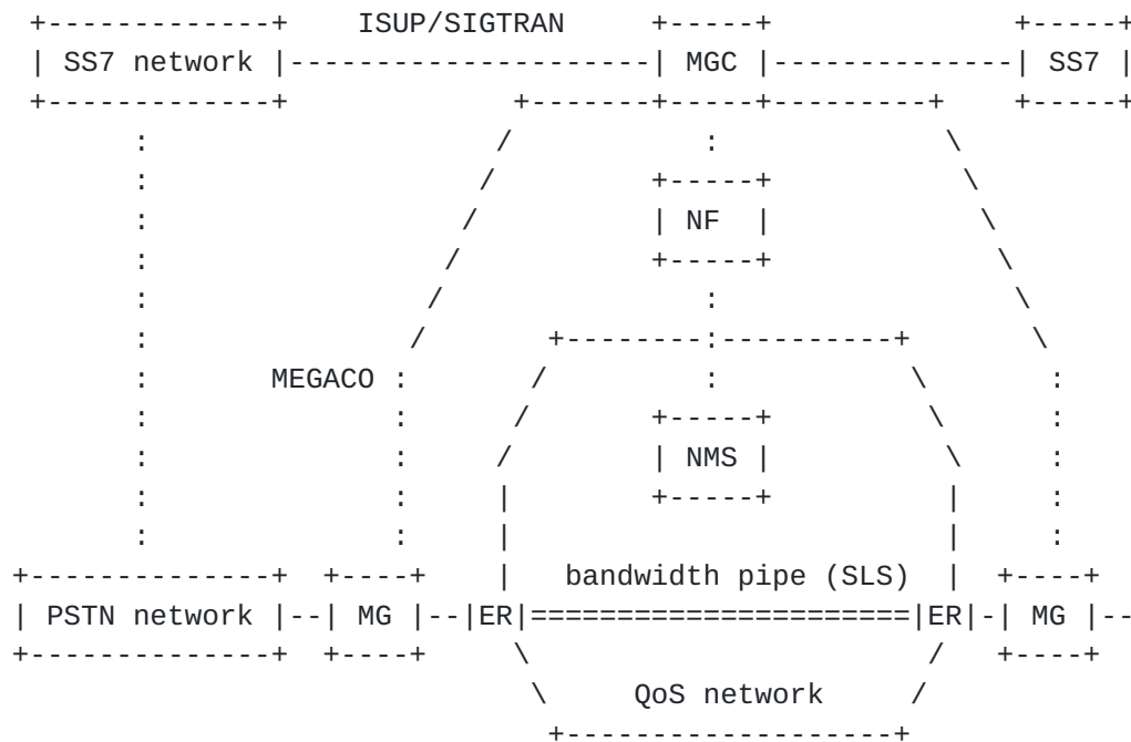
Figure 4: PSTN trunking gateway scenario
