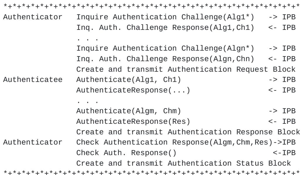
Figure 2. Authentication Message Flows
