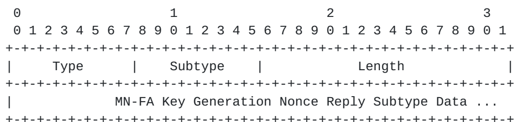
Figure 2: The Generalized Mobile IP MN-FA Key Generation Nonce Reply Extension
