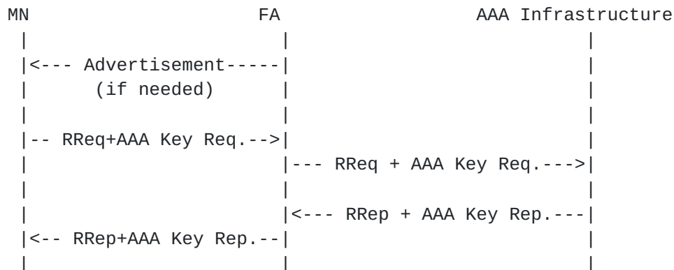
Figure 9: Message Flows for Requesting and Receiving Key Generation Nonce
