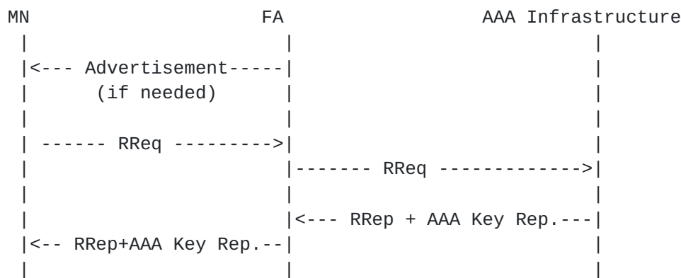
Figure 10: Message Flow for Receiving Unsolicited Key Generation Nonce
