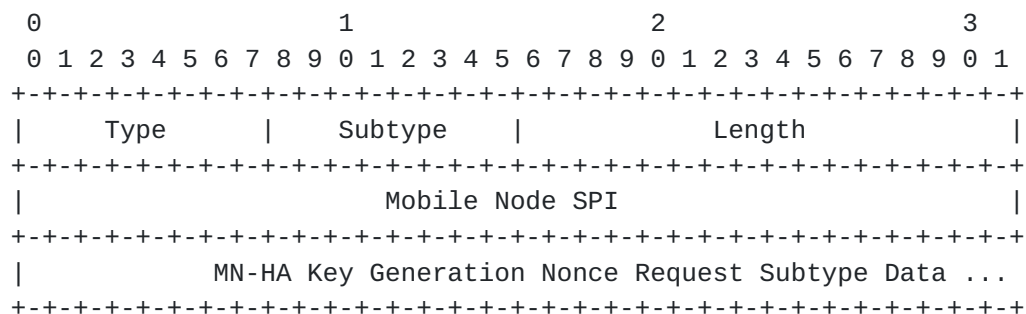
Figure 4: The Generalized Mobile IP MN-HA Key Generation Nonce Request Extension
