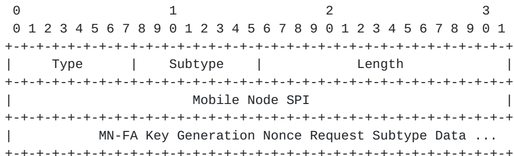
Figure 1: The Generalized Mobile IP MN-FA Key Generation Nonce Request Extension
