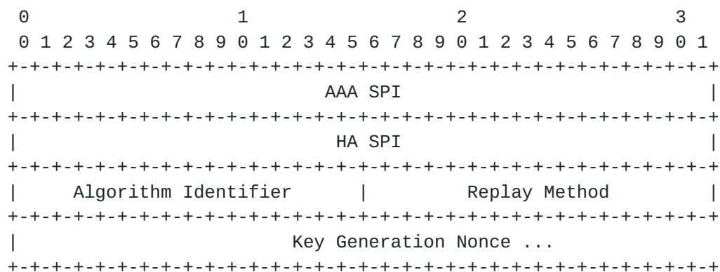
Figure 6: The MN-HA Key Generation Nonce From AAA Subtype-Specific Data
