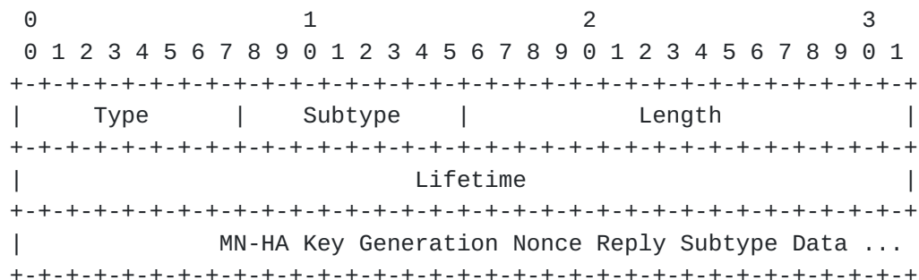
Figure 5: The Generalized Mobile IP MN-HA Key Generation Nonce Reply Extension
