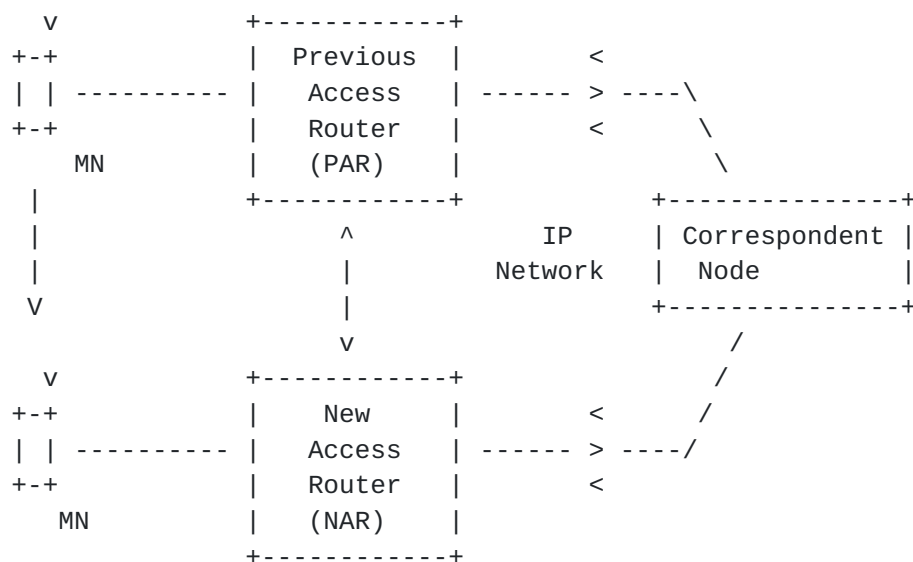
Figure 1: Reference Scenario for Handover
