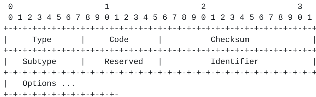
Figure 7: Handover Acknowledge (HACK) Message
