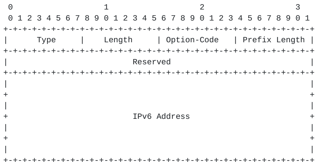
Figure 12: IPv6 Address Option
