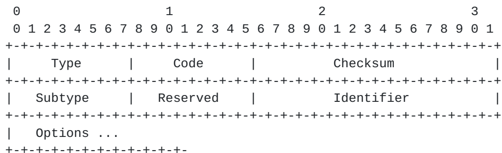
Figure 4: Router Solicitation for Proxy (RtSolPr) Message
