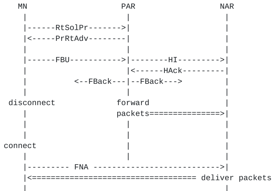
Figure 2: "Predictive" Fast Handover
