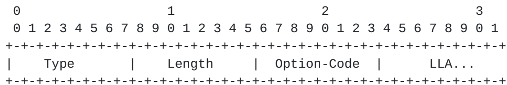
Figure 14: Link-Layer Address Option
