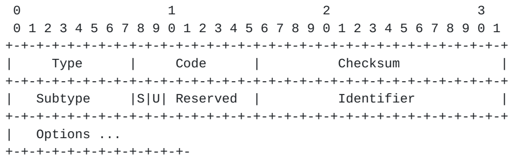
Figure 6: Handover Initiate (HI) Message
