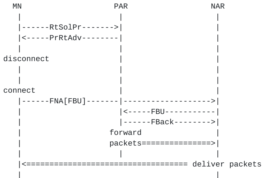
Figure 3: "Reactive" Fast Handover
