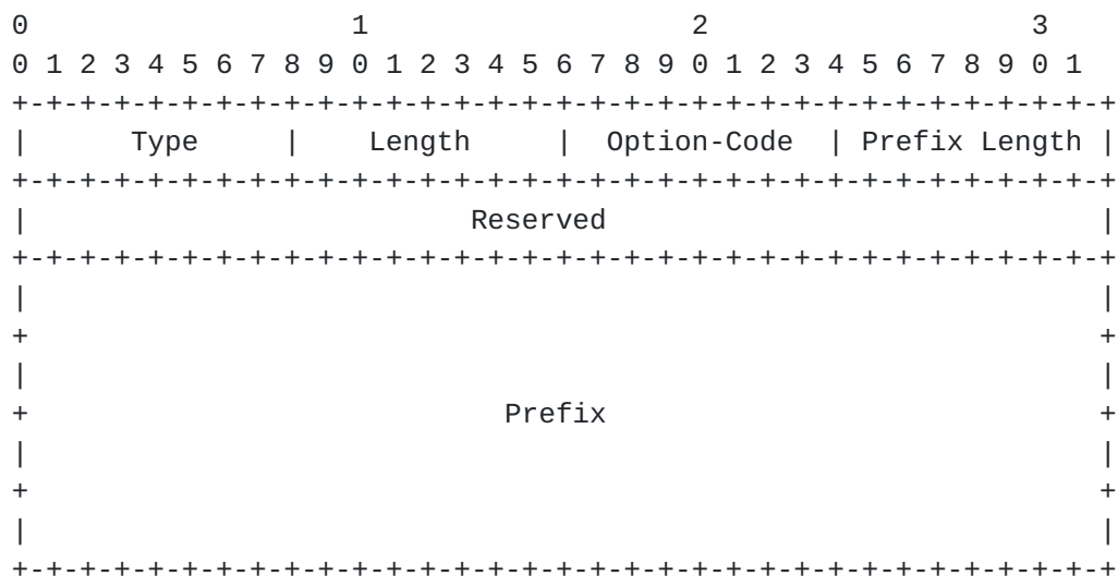
Figure 13: New Router Prefix Information Option
