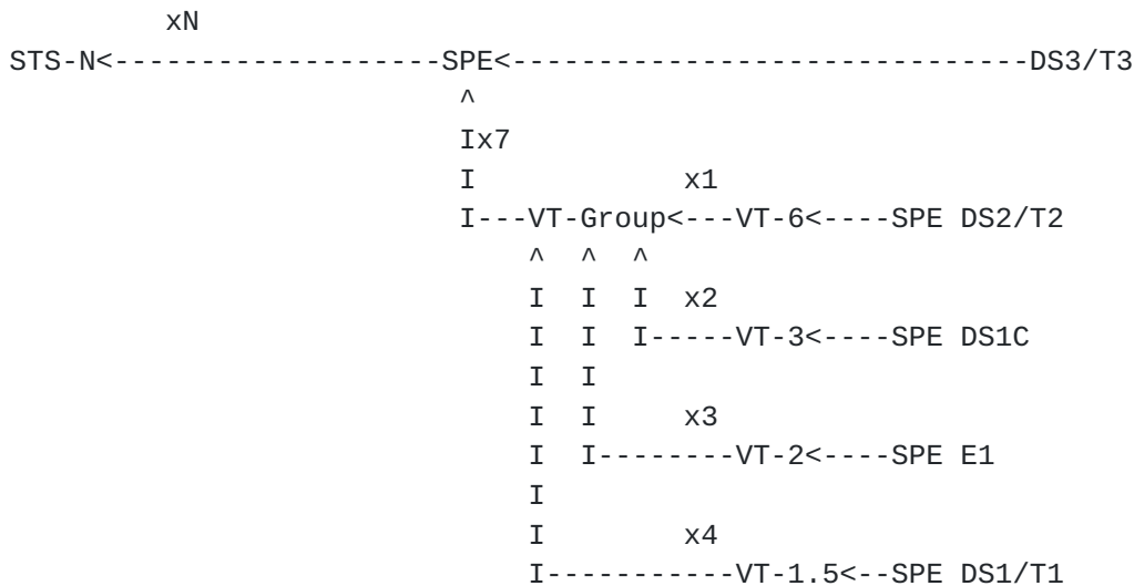
Figure 1. SDH and SONET multiplexing structure and typical Plesiochronous Digital Hierarchy (PDH) payload signals.
