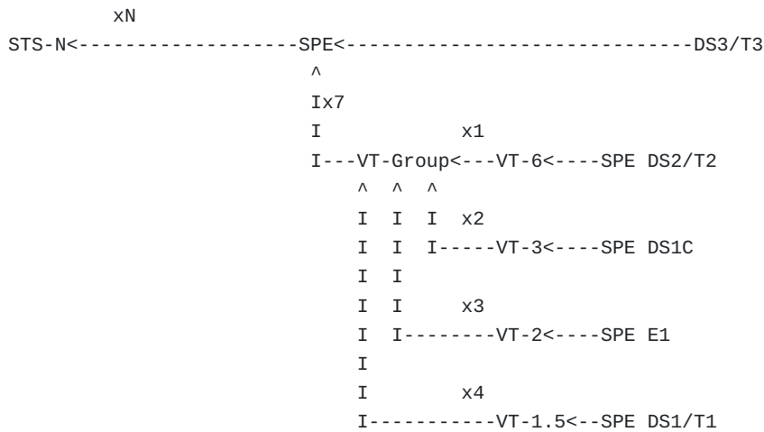
Figure 1. SDH and SONET multiplexing structure and typical Plesiochronous Digital Hierarchy (PDH) payload signals.
