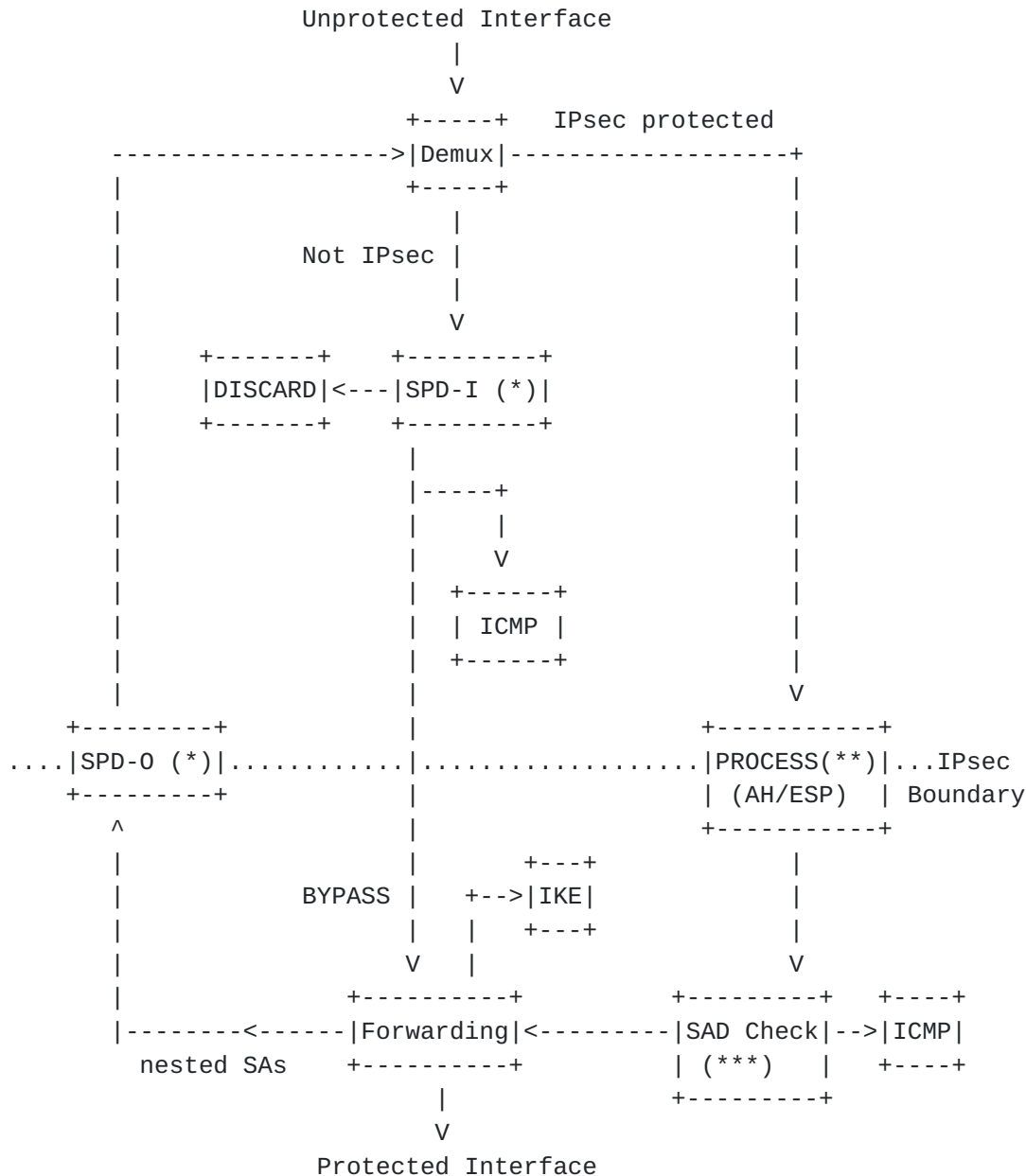
Figure 3. Processing Model for Inbound Traffic
