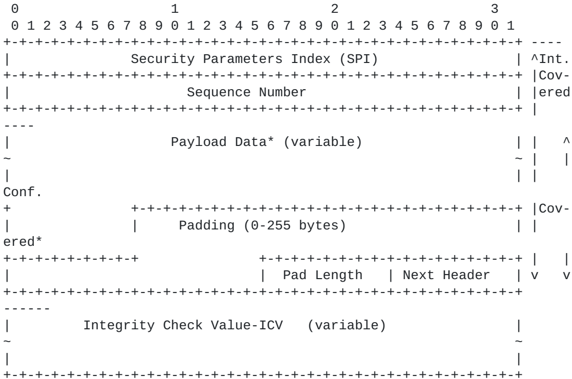
Figure 1. Top-Level Format of an ESP Packet
