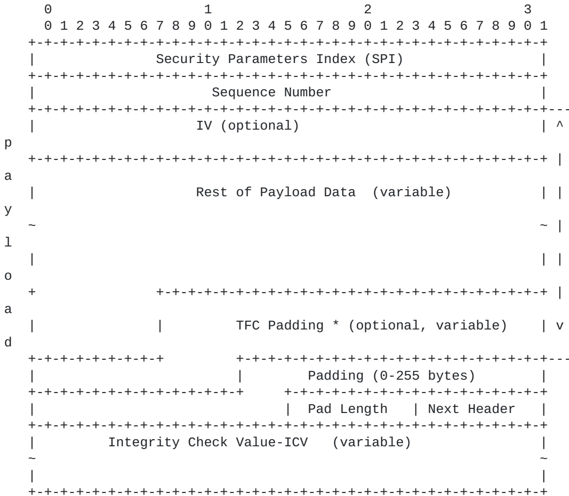
Figure 2. Substructure of Payload Data
