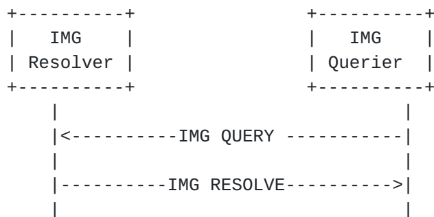
Figure 6: Query/Resolve Sequence Example
