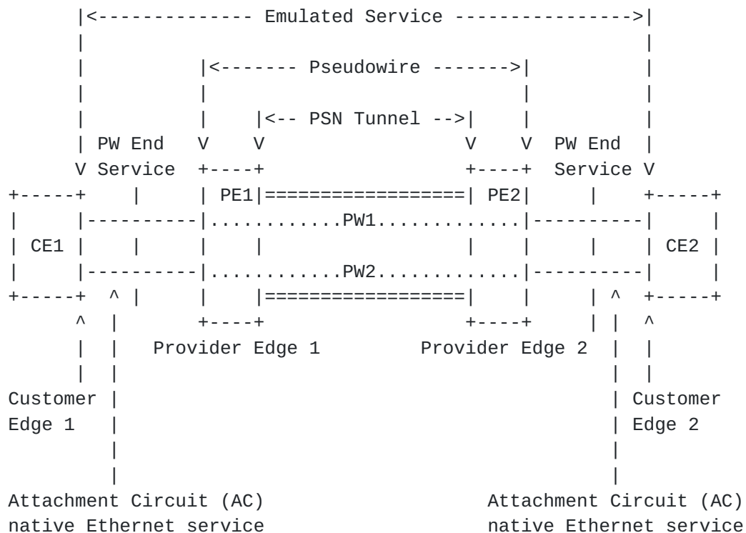
Figure 1: PWE3 Ethernet/VLAN Interface Reference Configuration
