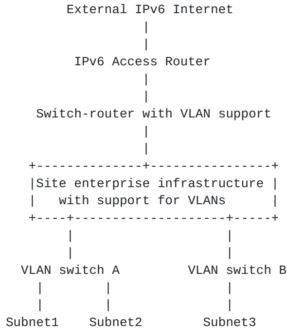
Figure 1: IPv6 deployment using VLANs (physical diagram)
