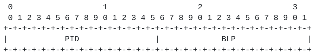
Figure 4: Syntax for the Generic NACK message
