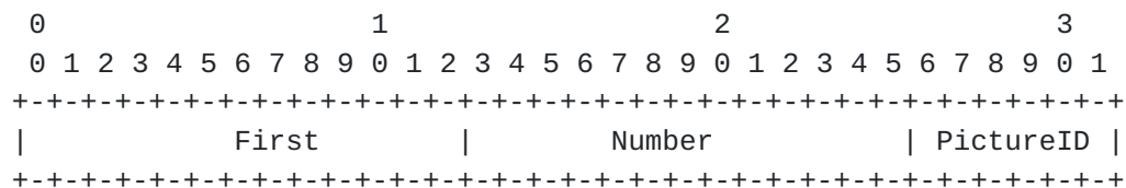
Figure 6: Syntax of the Slice Loss Indication (SLI)
