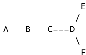
Figure 1. An example P2MP tree where the data path and control plane state branch at C, but the topology branches at D.
