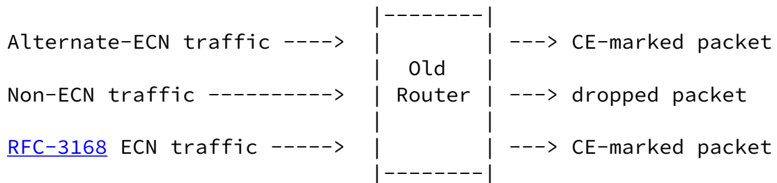
Figure 1: Alternate-ECN traffic, an old router, using RFC-3168 ECN, that is congested and ready to drop or mark the arriving packet.
