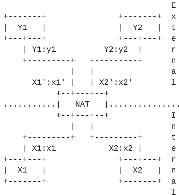
Port Assignment
