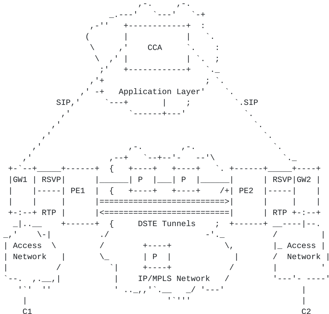
Figure B1. Integration of SIP Resource Management and RSVP Aggregation over MPLS TE Tunnels
