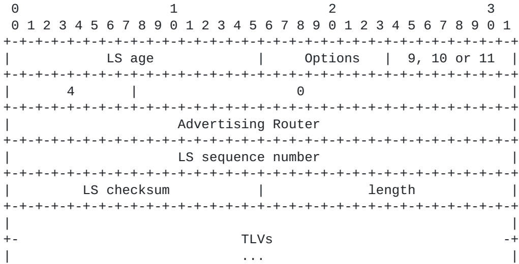
OSPFv2 Router Information Opaque LSA
