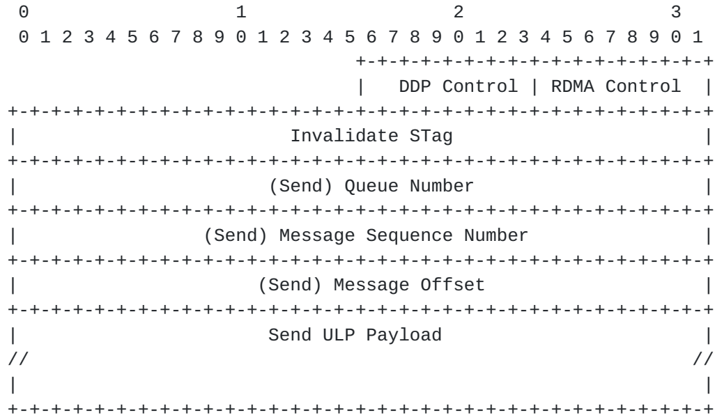
Figure 15: Send with Invalidate and Send with SE and Invalidate, DDP Segment Format
