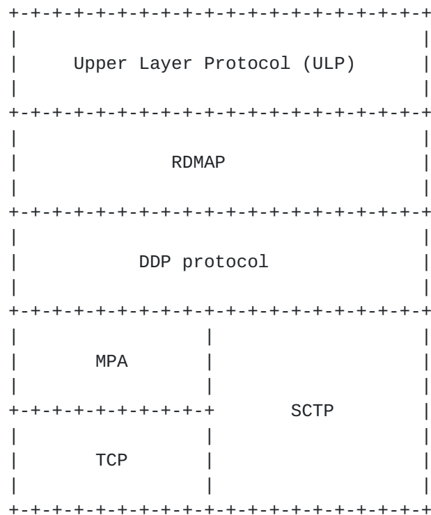
Figure 1: RDMA Layering
