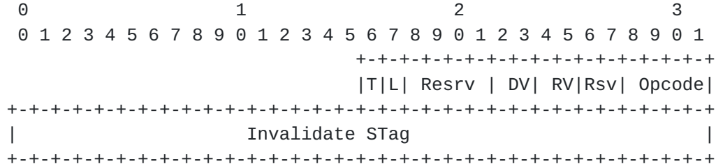
Figure 3: DDP Control, RDMAP Control, and Invalidate STag Fields
