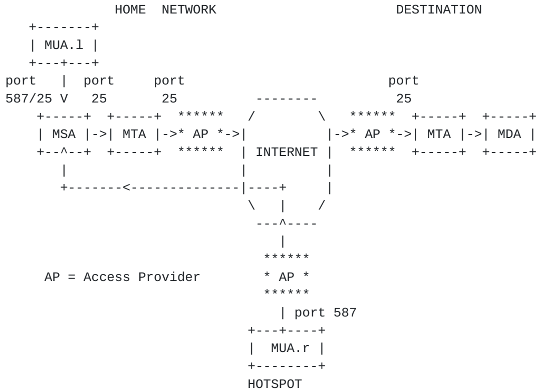
Figure 1: Example of Port 587 Usage via Internet
