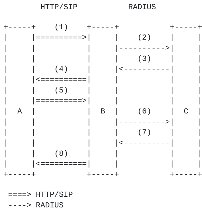
Figure 2: HTTP Digest over RADIUS
